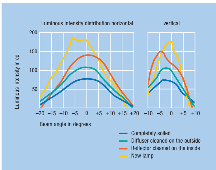
Effect of soiling and bulb blackening on the signal luminous intensity of a mains voltage lamp
