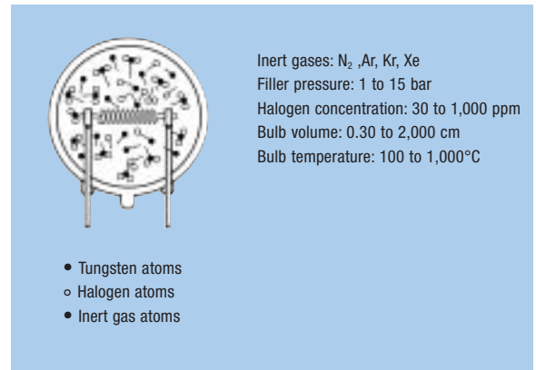
Fig. 3: Halogen lamp with halogen cycle
