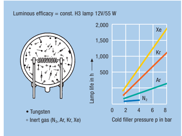
Fig. 2: Gas-filled lamp showing lamp life as a function of cold filler pressure and type of gas
