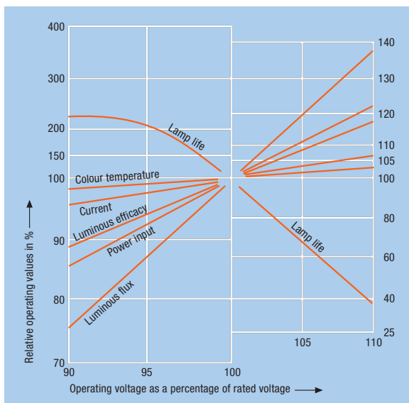
Fig. 2: Operational characteristics of halogen lamps (referred to L_{max} \leq 1,000 h)
