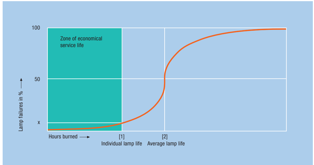
Lamp life
