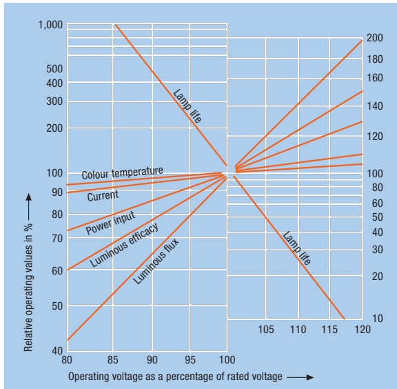
Fig. 1: Operational characteristics of gas-filled lamps
