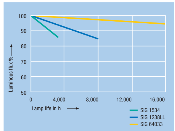
Fig. 4: Residual luminous flux for different signal lamps (HV/NV/HAL)
