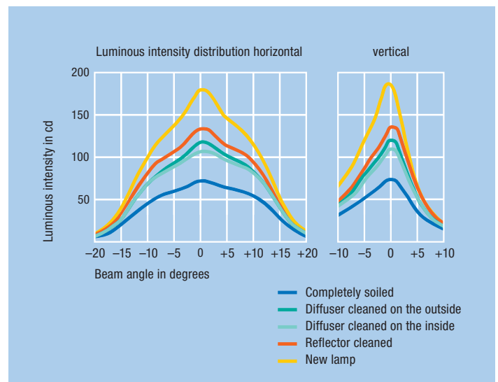
Effect of soiling and bulb blackening on the signal luminous intensity of a low-voltage lamp
