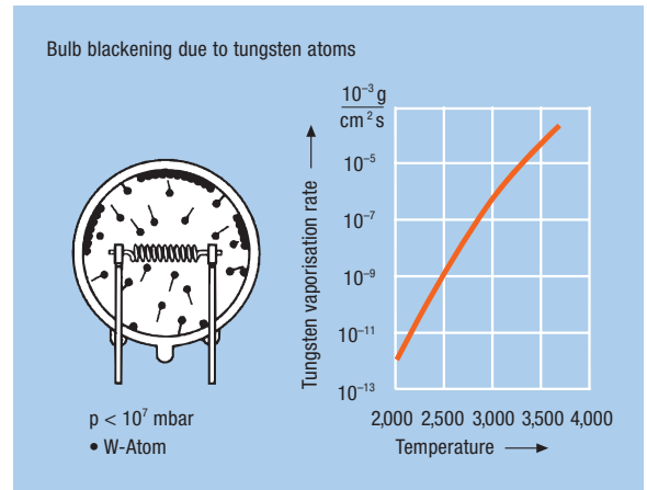
Fig. 1: Vacuum lamps with tungsten vaporisation rate
